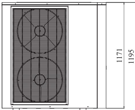
Outdoor —— NP13-V7-S
