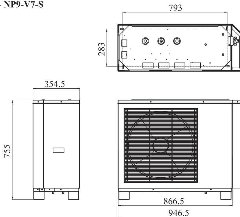
Outdoor — NP9-V7-S
